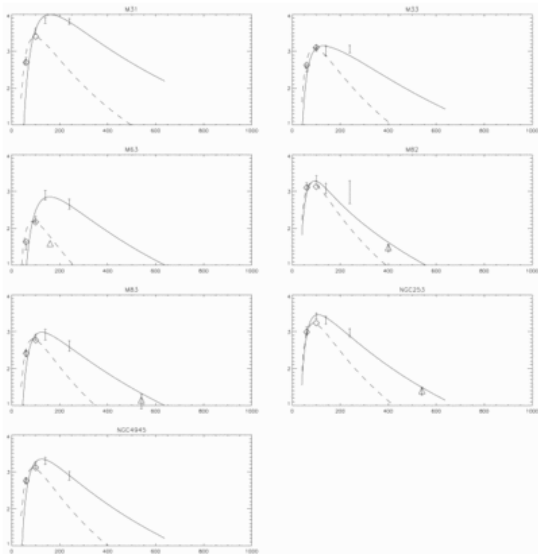
Fig. 4. from A Study of External Galaxies Detected by the COBE Diffuse Infrared Background Experiment Odenwald, Newmark, & Smoot 1998 ApJ 500 554 doi:10.1086/305737 https://dx.doi.org/10.1086/305737 © 1998. The American Astronomical Society. All rights reserved. Printed in U.S.A.
