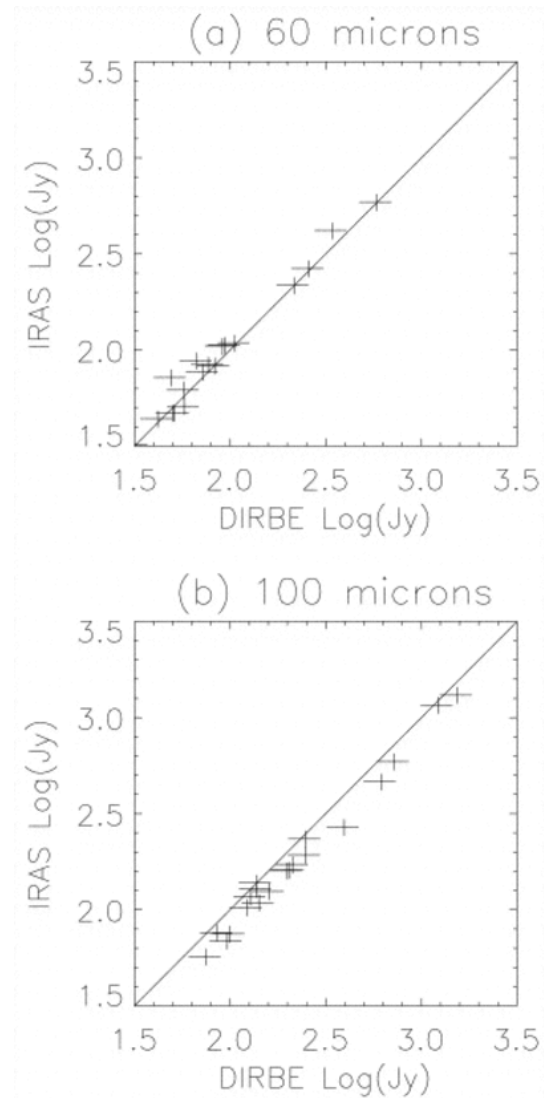
Fig. 2. from A Study of External Galaxies Detected by the COBE Diffuse Infrared Background Experiment Odenwald, Newmark, & Smoot 1998 ApJ 500 554 doi:10.1086/305737 https://dx.doi.org/10.1086/305737 © 1998. The American Astronomical Society. All rights reserved. Printed in U.S.A.
