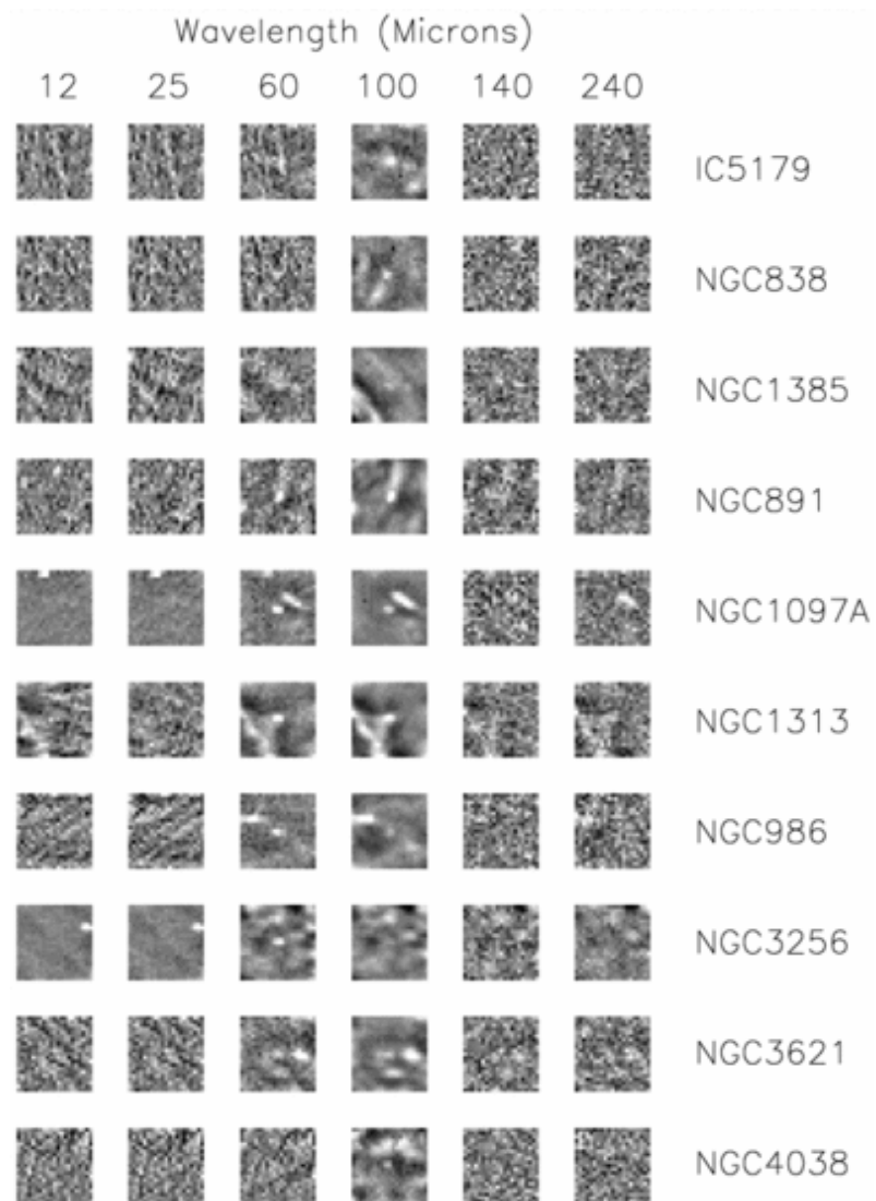
Fig. 1. from A Study of External Galaxies Detected by the COBE Diffuse Infrared Background Experiment Odenwald, Newmark, & Smoot 1998 ApJ 500 554 doi:10.1086/305737 https://dx.doi.org/10.1086/305737 © 1998. The American Astronomical Society. All rights reserved. Printed in U.S.A.
