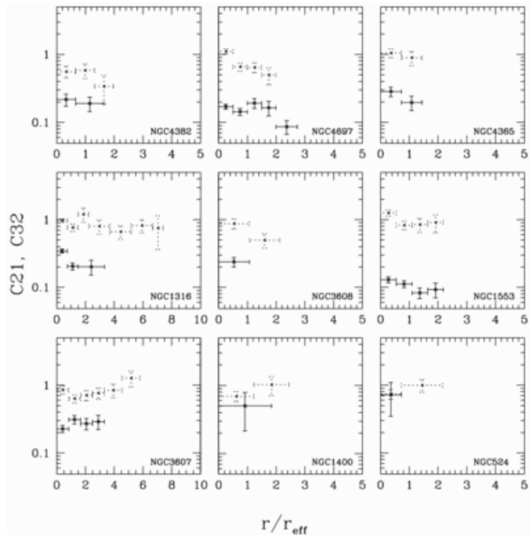
Fig. 7. from ROSAT XRay Colors and Emission Mechanisms in EarlyType Galaxies Irwin & Sarazin 1998 ApJ 499 650 doi:10.1086/305666 https://dx.doi.org/10.1086/305666 © 1998. The American Astronomical Society. All rights reserved. Printed in U.S.A.
