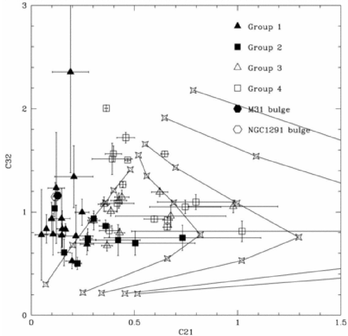
Fig. 6. from ROSAT XRay Colors and Emission Mechanisms in EarlyType Galaxies Irwin & Sarazin 1998 ApJ 499 650 doi:10.1086/305666 https://dx.doi.org/10.1086/305666 © 1998. The American Astronomical Society. All rights reserved. Printed in U.S.A.
