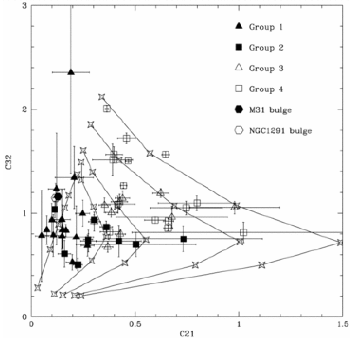
Fig. 5. from ROSAT XRay Colors and Emission Mechanisms in EarlyType Galaxies Irwin & Sarazin 1998 ApJ 499 650 doi:10.1086/305666 https://dx.doi.org/10.1086/305666 © 1998. The American Astronomical Society. All rights reserved. Printed in U.S.A.
