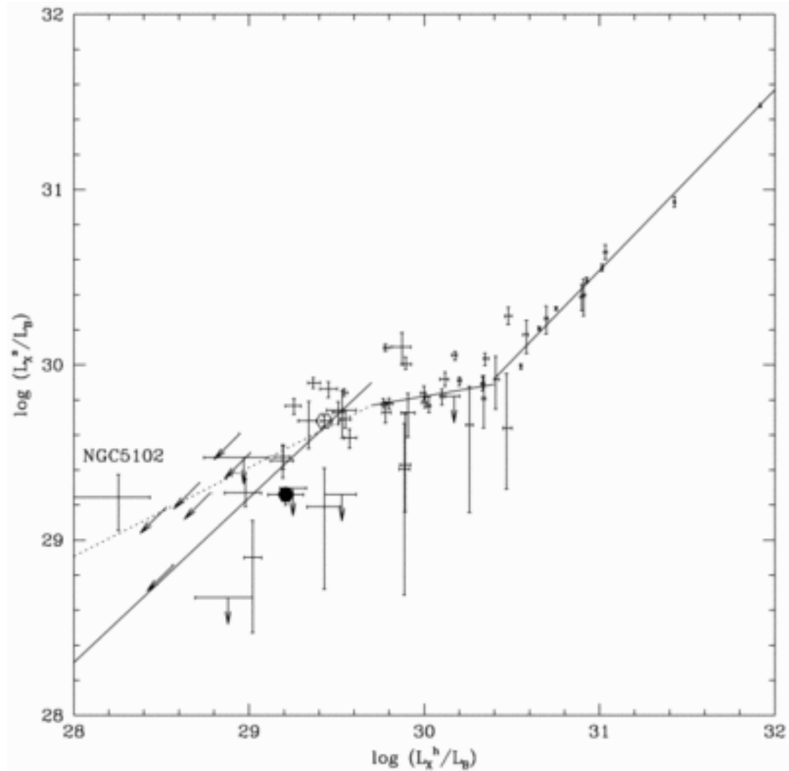
Fig. 3. from ROSAT XRay Colors and Emission Mechanisms in EarlyType Galaxies Irwin & Sarazin 1998 ApJ 499 650 doi:10.1086/305666 https://dx.doi.org/10.1086/305666 © 1998. The American Astronomical Society. All rights reserved. Printed in U.S.A.
