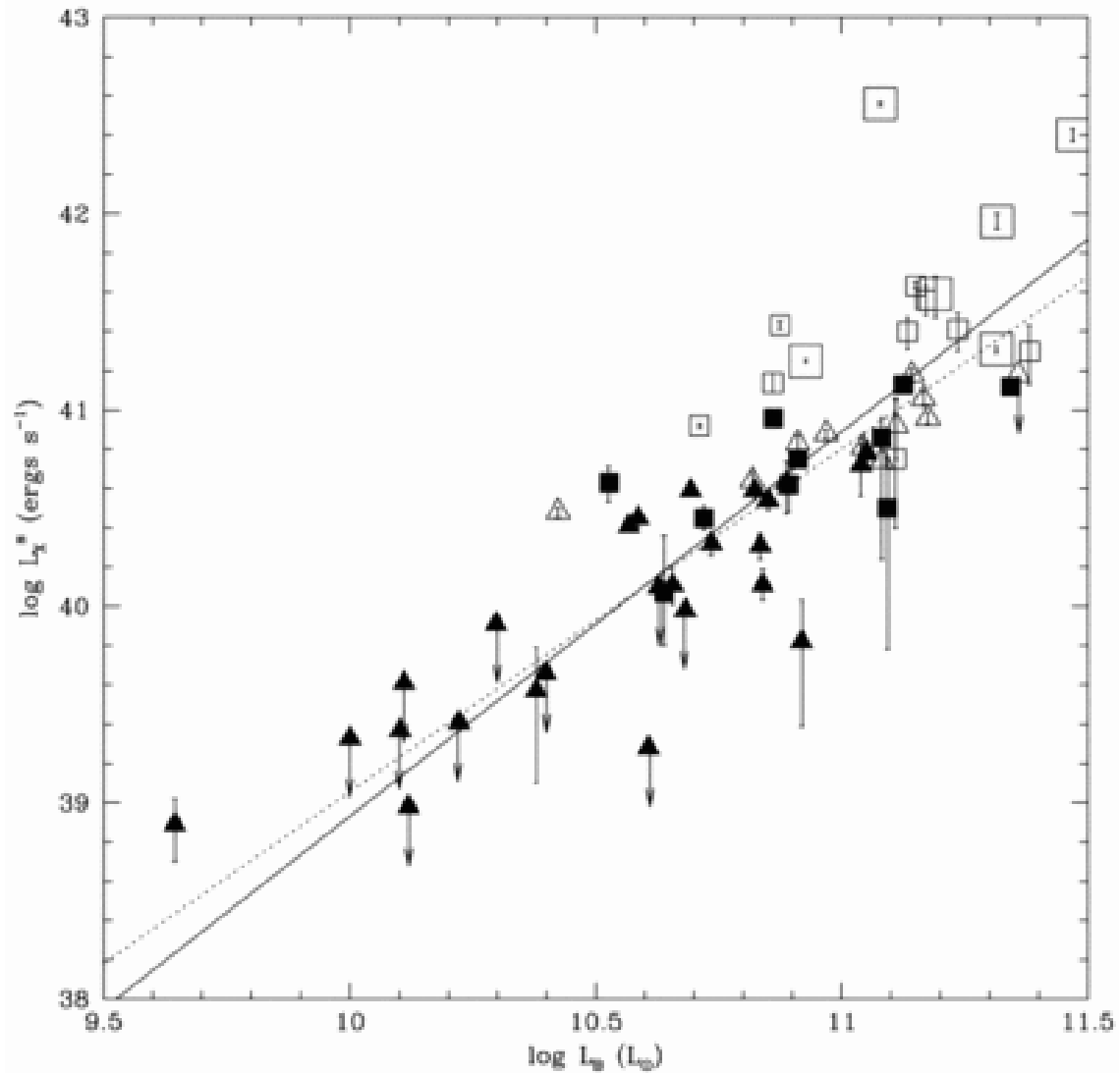
Fig. 2. from ROSAT XRay Colors and Emission Mechanisms in EarlyType Galaxies Irwin & Sarazin 1998 ApJ 499 650 doi:10.1086/305666 https://dx.doi.org/10.1086/305666 © 1998. The American Astronomical Society. All rights reserved. Printed in U.S.A.
