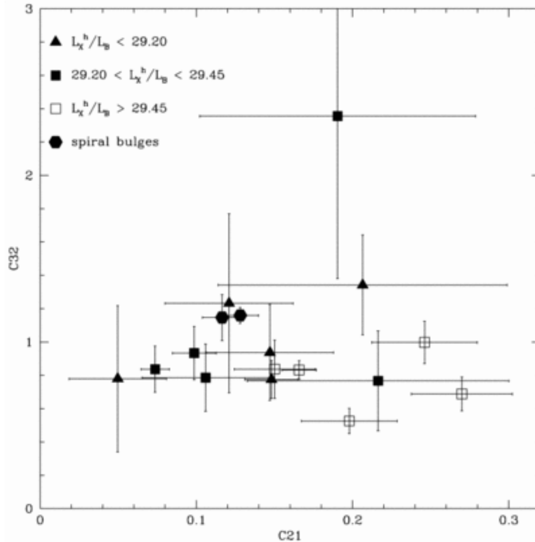
Fig. 11. from ROSAT XRay Colors and Emission Mechanisms in EarlyType Galaxies Irwin & Sarazin 1998 ApJ 499 650 doi:10.1086/305666 https://dx.doi.org/10.1086/305666 © 1998. The American Astronomical Society. All rights reserved. Printed in U.S.A.
