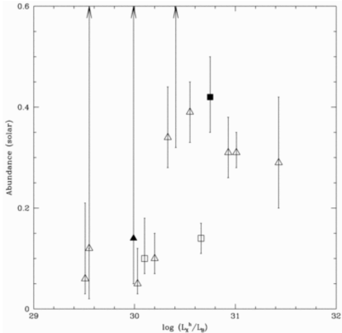
Fig. 10. from ROSAT XRay Colors and Emission Mechanisms in EarlyType Galaxies Irwin & Sarazin 1998 ApJ 499 650 doi:10.1086/305666 https://dx.doi.org/10.1086/305666 © 1998. The American Astronomical Society. All rights reserved. Printed in U.S.A.
