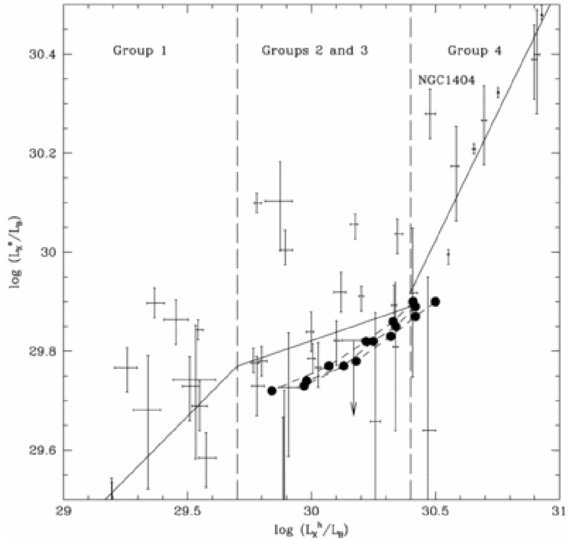
Fig. 9. from ROSAT XRay Colors and Emission Mechanisms in EarlyType Galaxies Irwin & Sarazin 1998 ApJ 499 650 doi:10.1086/305666 https://dx.doi.org/10.1086/305666 © 1998. The American Astronomical Society. All rights reserved. Printed in U.S.A.
