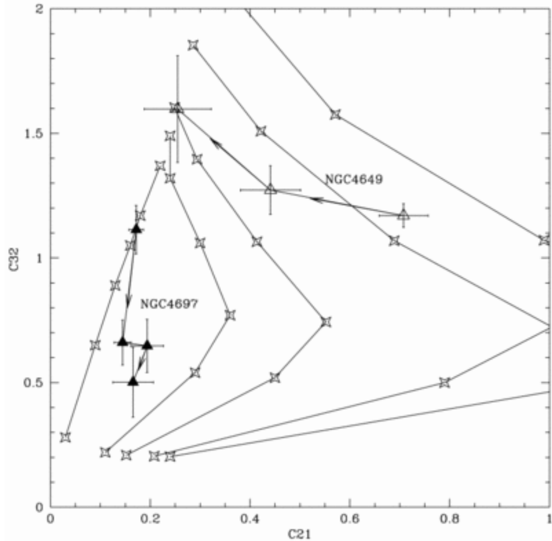
Fig. 8. from ROSAT XRay Colors and Emission Mechanisms in EarlyType Galaxies Irwin & Sarazin 1998 ApJ 499 650 doi:10.1086/305666 https://dx.doi.org/10.1086/305666 © 1998. The American Astronomical Society. All rights reserved. Printed in U.S.A.
