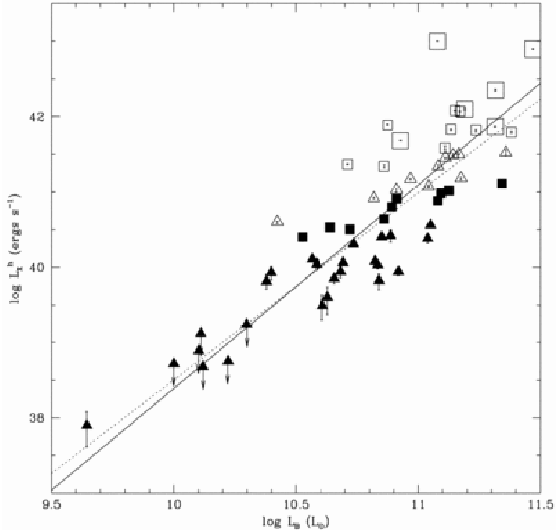
Fig. 1. from ROSAT XRay Colors and Emission Mechanisms in EarlyType Galaxies Irwin & Sarazin 1998 ApJ 499 650 doi:10.1086/305666 https://dx.doi.org/10.1086/305666 © 1998. The American Astronomical Society. All rights reserved. Printed in U.S.A.
