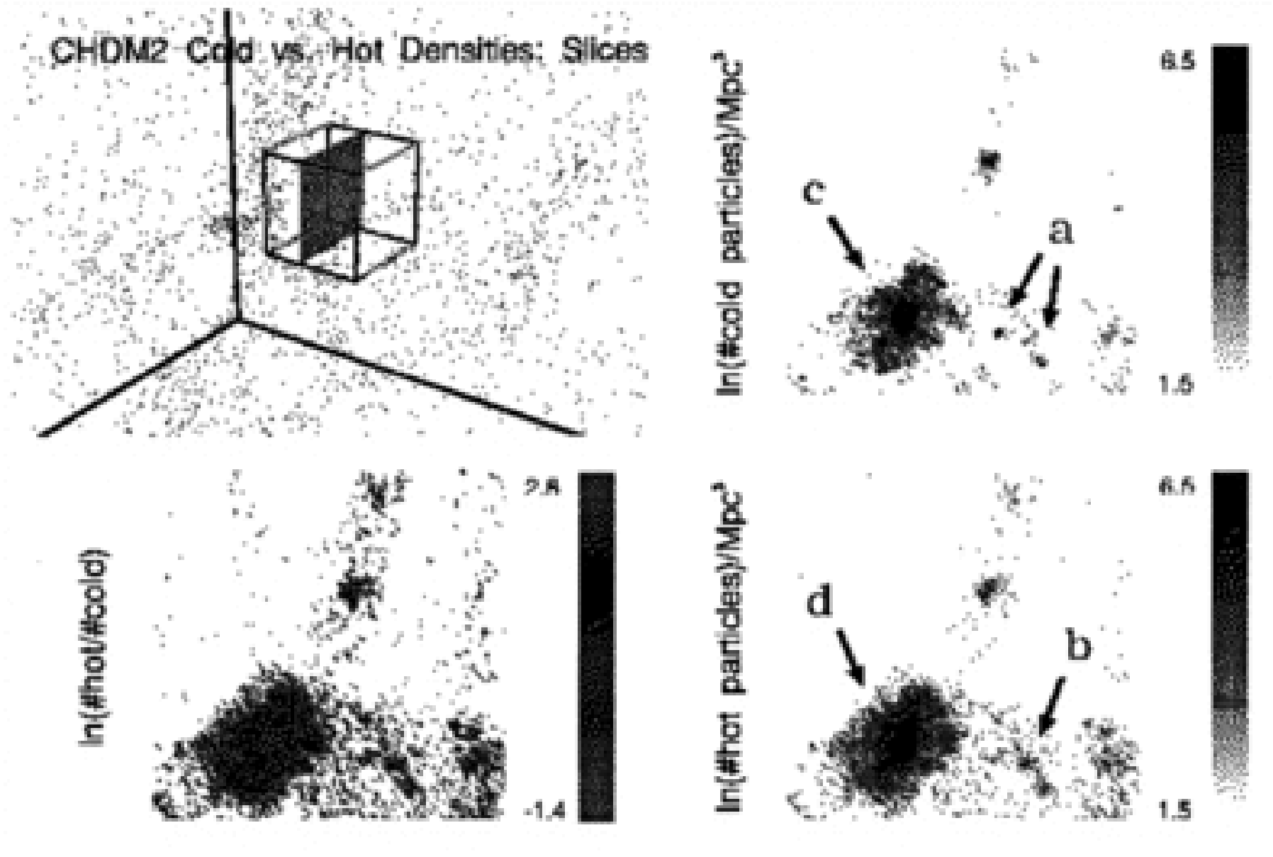
Fig. 4. from Visualization of Cold + Hot and Cold Dark Matter Cosmologies versus CfA1 Data Brodbeck et al. 1998 ApJ 495 1 doi:10.1086/305250 https://dx.doi.org/10.1086/305250 © 1998. The American Astronomical Society. All rights reserved. Printed in U.S.A.
