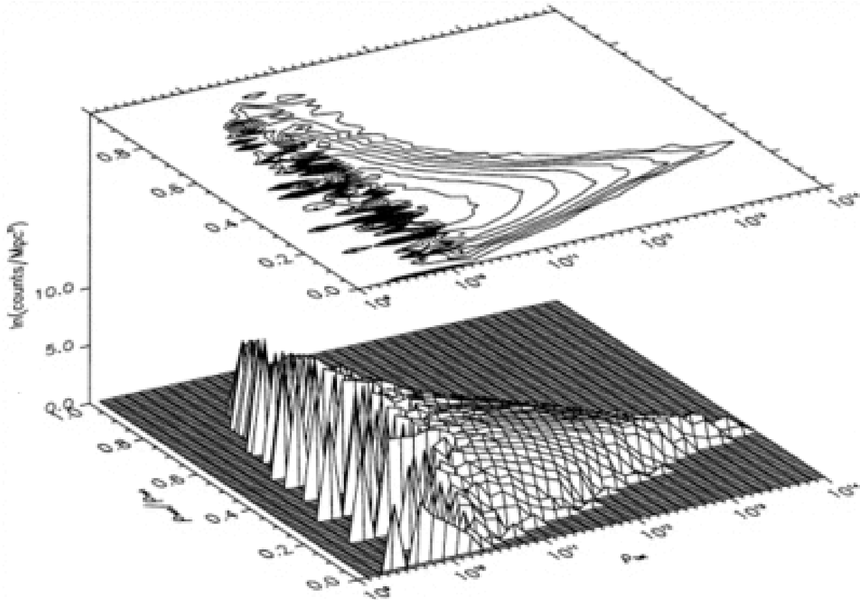
Fig. 3. from Visualization of Cold + Hot and Cold Dark Matter Cosmologies versus CfA1 Data Brodbeck et al. 1998 ApJ 495 1 doi:10.1086/305250 https://dx.doi.org/10.1086/305250 © 1998. The American Astronomical Society. All rights reserved. Printed in U.S.A.
