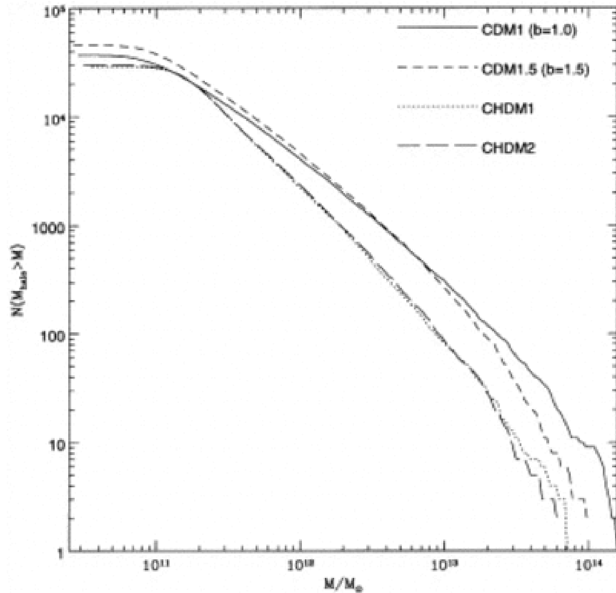
Fig. 1. from Visualization of Cold + Hot and Cold Dark Matter Cosmologies versus CfA1 Data Brodbeck et al. 1998 ApJ 495 1 doi:10.1086/305250 https://dx.doi.org/10.1086/305250 © 1998. The American Astronomical Society. All rights reserved. Printed in U.S.A.
