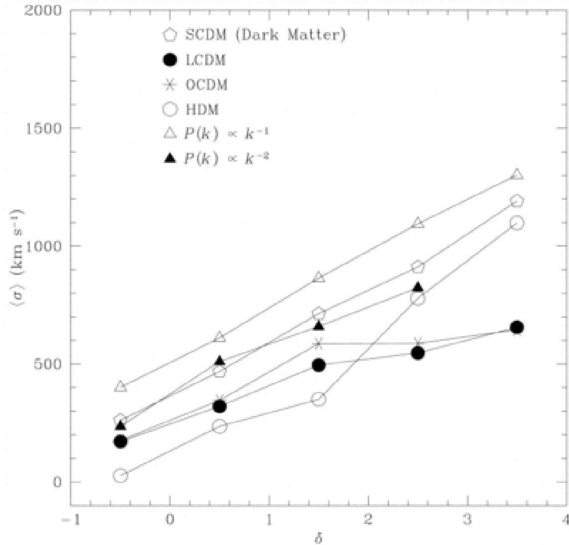
Fig. 6. from The Galaxy Pairwise Velocity Dispersion as a Function of Local Density Strauss, Ostriker, & Cen 1998 ApJ 494 20 doi:10.1086/305211 https://dx.doi.org/10.1086/305211 © 1998. The American Astronomical Society. All rights reserved. Printed in U.S.A.
