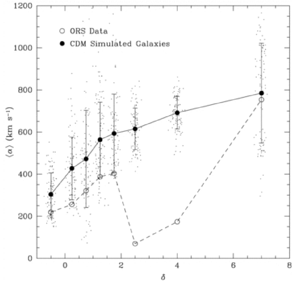
Fig. 4. from The Galaxy Pairwise Velocity Dispersion as a Function of Local Density Strauss, Ostriker, & Cen 1998 ApJ 494 20 doi:10.1086/305211 https://dx.doi.org/10.1086/305211 © 1998. The American Astronomical Society. All rights reserved. Printed in U.S.A.
