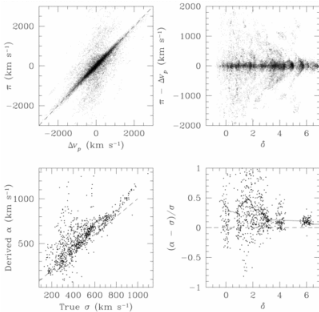
Fig. 3. from The Galaxy Pairwise Velocity Dispersion as a Function of Local Density Strauss, Ostriker, & Cen 1998 ApJ 494 20 doi:10.1086/305211 https://dx.doi.org/10.1086/305211 © 1998. The American Astronomical Society. All rights reserved. Printed in U.S.A.
