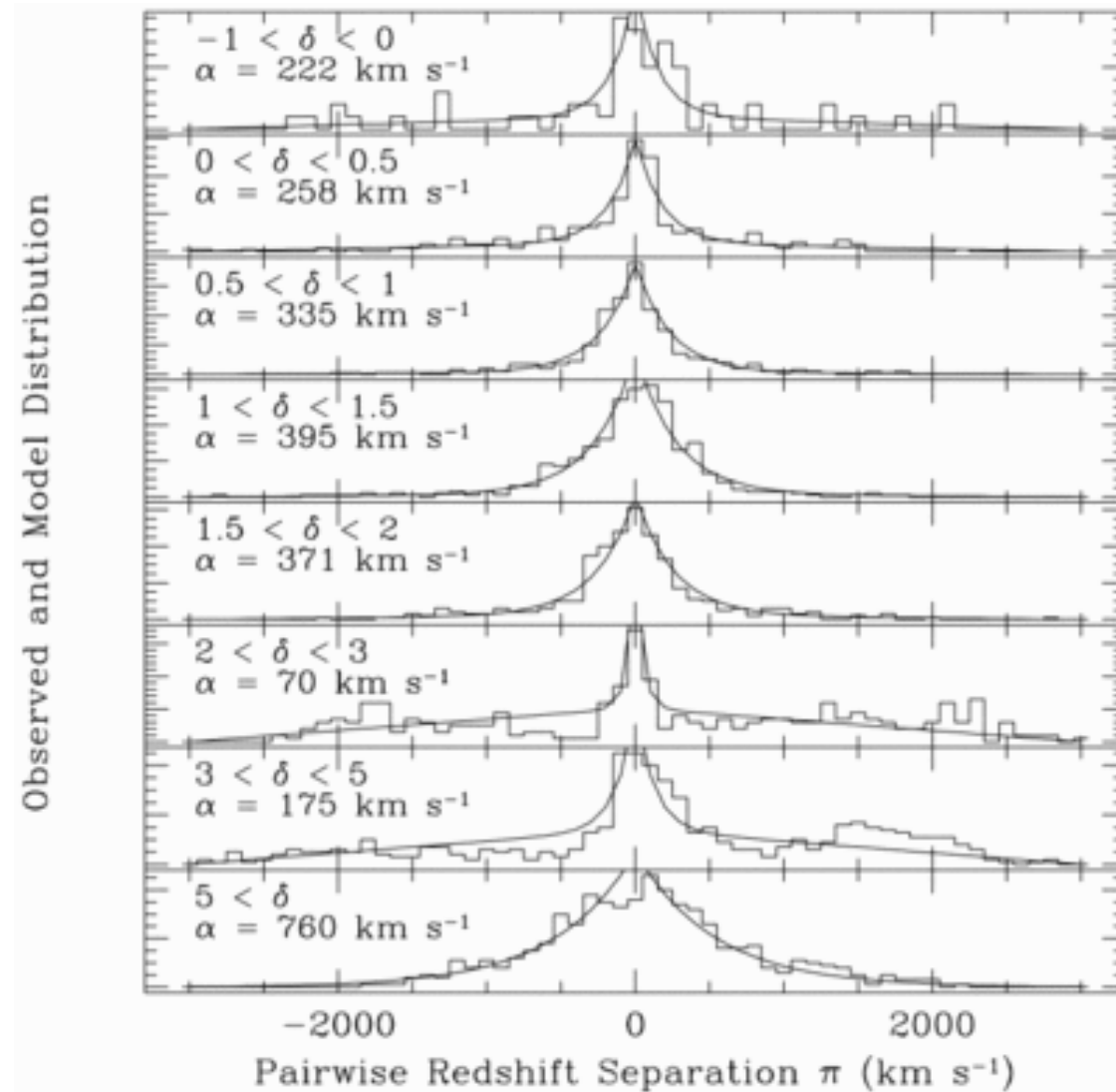
Fig. 2. from The Galaxy Pairwise Velocity Dispersion as a Function of Local Density Strauss, Ostriker, & Cen 1998 ApJ 494 20 doi:10.1086/305211 https://dx.doi.org/10.1086/305211 © 1998. The American Astronomical Society. All rights reserved. Printed in U.S.A.
