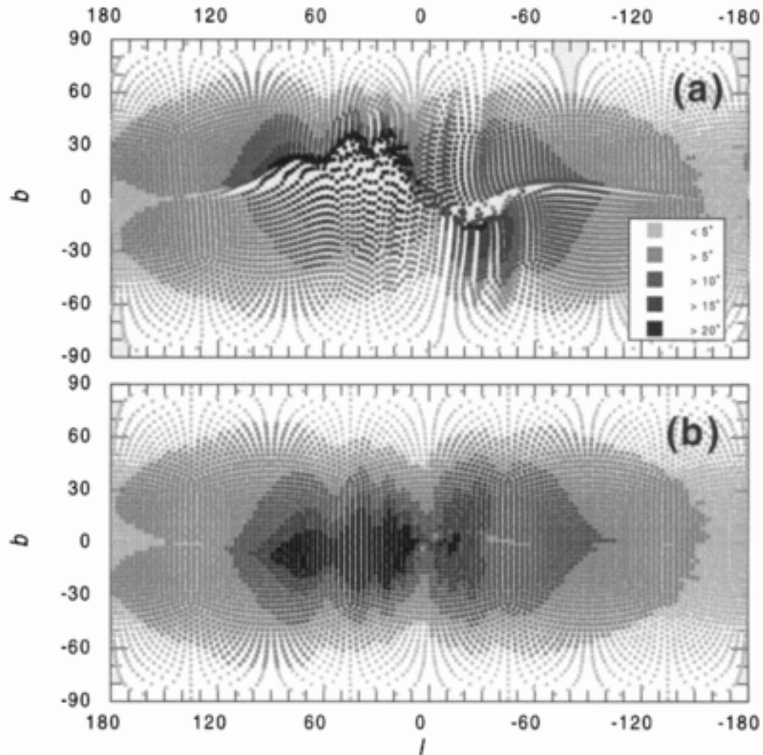
Fig. 1. from Deflection of Ultra-HighEnergy Cosmic Rays by the Galactic Magnetic Field: From the Sources to the Detector Medina Tanco, de Gouveia Dal Pino, & Horvath 1998 ApJ 492 200 doi:10.1086/305044 https://dx.doi.org/10.1086/305044 © 1998. The American Astronomical Society. All rights reserved. Printed in U.S.A.
