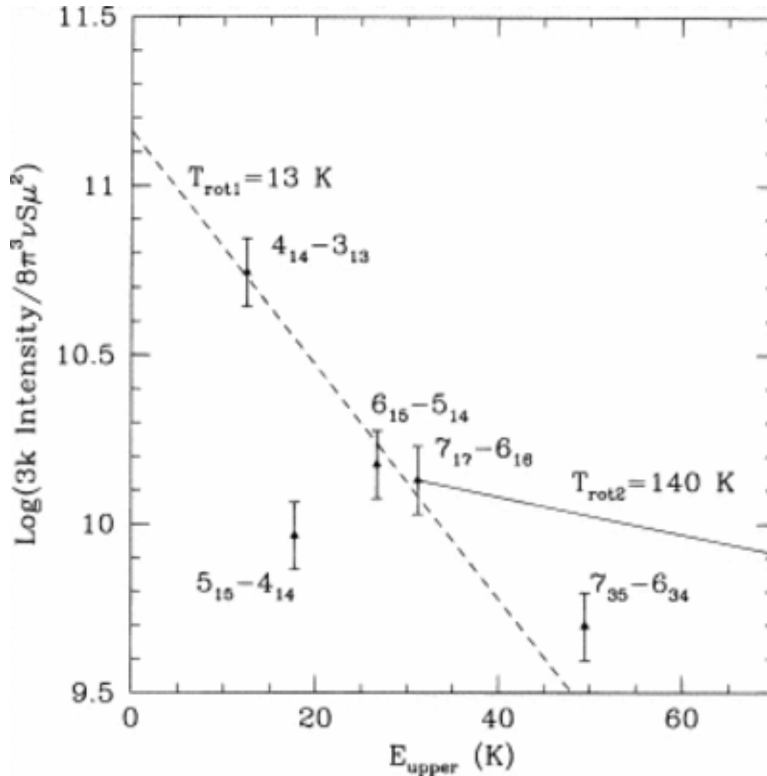
Fig. 3. from A Search for Vibrationally Excited SiC2 3 = 1 toward IRC+10216 Gensheimer & Snyder 1997 ApJ 490 819 doi:10.1086/304916 https://dx.doi.org/10.1086/304916 © 1997. The American Astronomical Society. All rights reserved. Printed in U.S.A.
