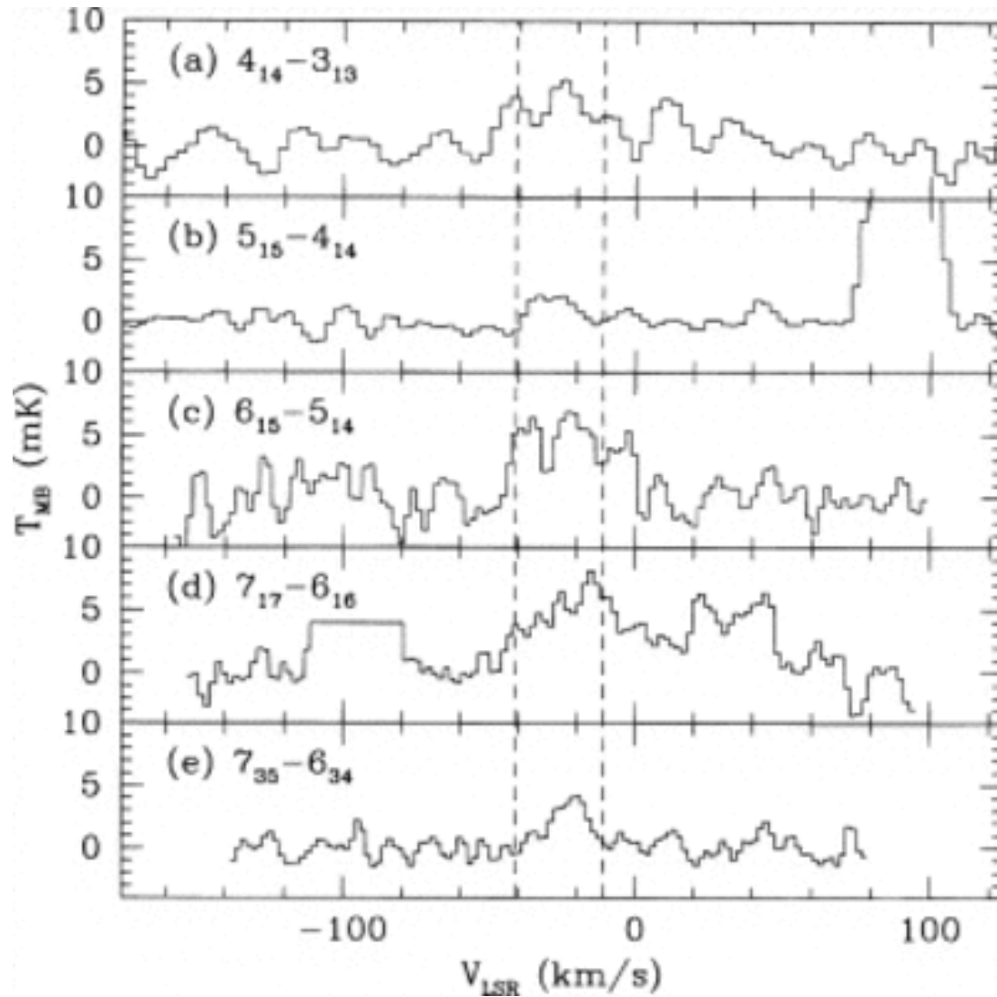
Fig. 1. from A Search for Vibrationally Excited SiC2 3 = 1 toward IRC+10216 Gensheimer & Snyder 1997 ApJ 490 819 doi:10.1086/304916 https://dx.doi.org/10.1086/304916 © 1997. The American Astronomical Society. All rights reserved. Printed in U.S.A.
