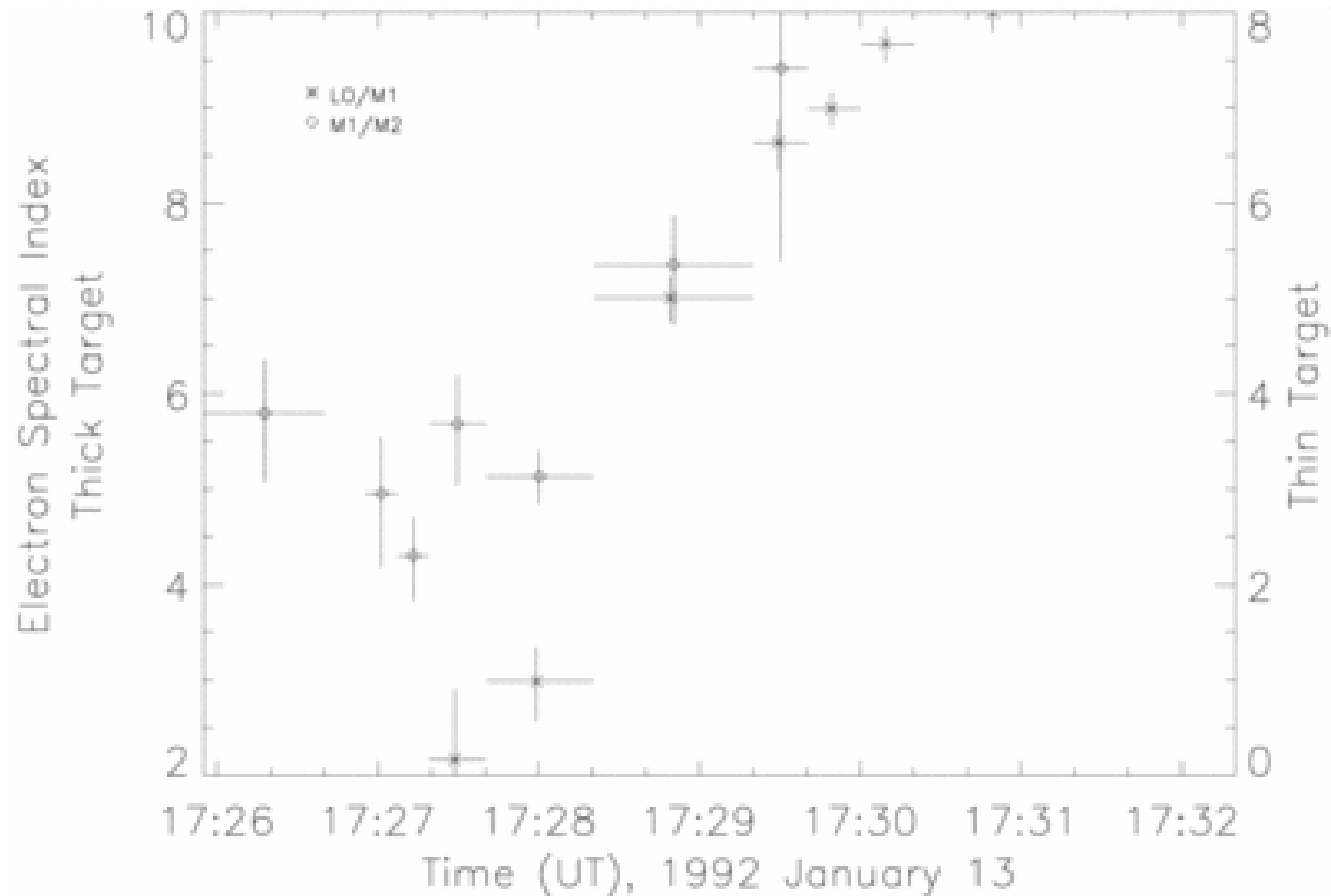
Fig. 9. from A Spectral Analysis of the Masuda Flare Using Yohkoh Hard XRay Telescope Pixon Reconstruction Alexander & Metcalf 1997 ApJ 489 442 doi:10.1086/304762 https://dx.doi.org/10.1086/304762 © 1997. The American Astronomical Society. All rights reserved. Printed in U.S.A.
