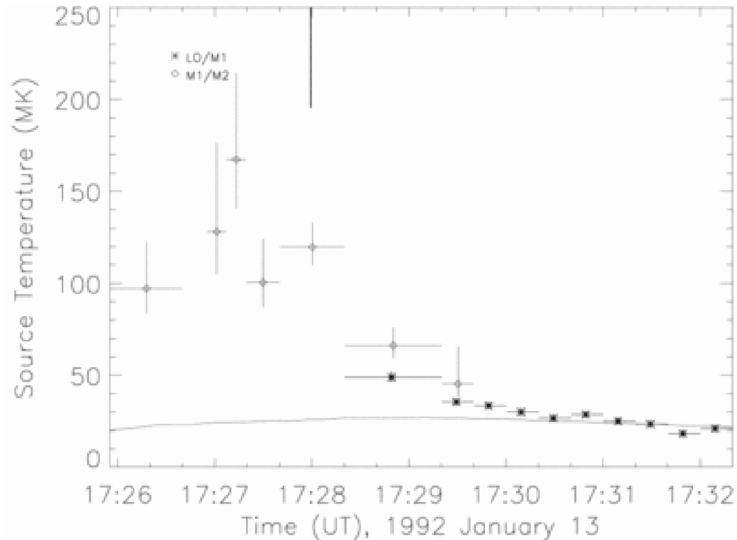
Fig. 8. from A Spectral Analysis of the Masuda Flare Using Yohkoh Hard XRay Telescope Pixon Reconstruction Alexander & Metcalf 1997 ApJ 489 442 doi:10.1086/304762 https://dx.doi.org/10.1086/304762 © 1997. The American Astronomical Society. All rights reserved. Printed in U.S.A.
