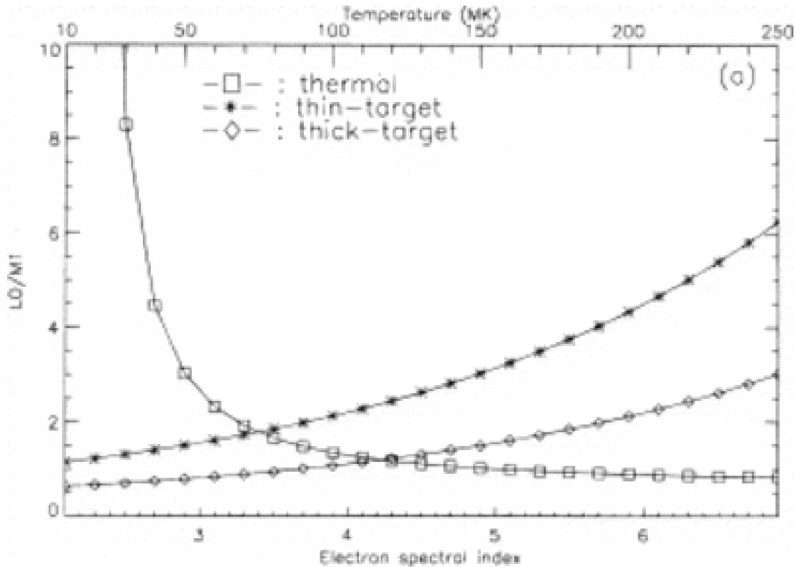
Fig. 7. from A Spectral Analysis of the Masuda Flare Using Yohkoh Hard XRay Telescope Pixon Reconstruction Alexander & Metcalf 1997 ApJ 489 442 doi:10.1086/304762 https://dx.doi.org/10.1086/304762 © 1997. The American Astronomical Society. All rights reserved. Printed in U.S.A.
