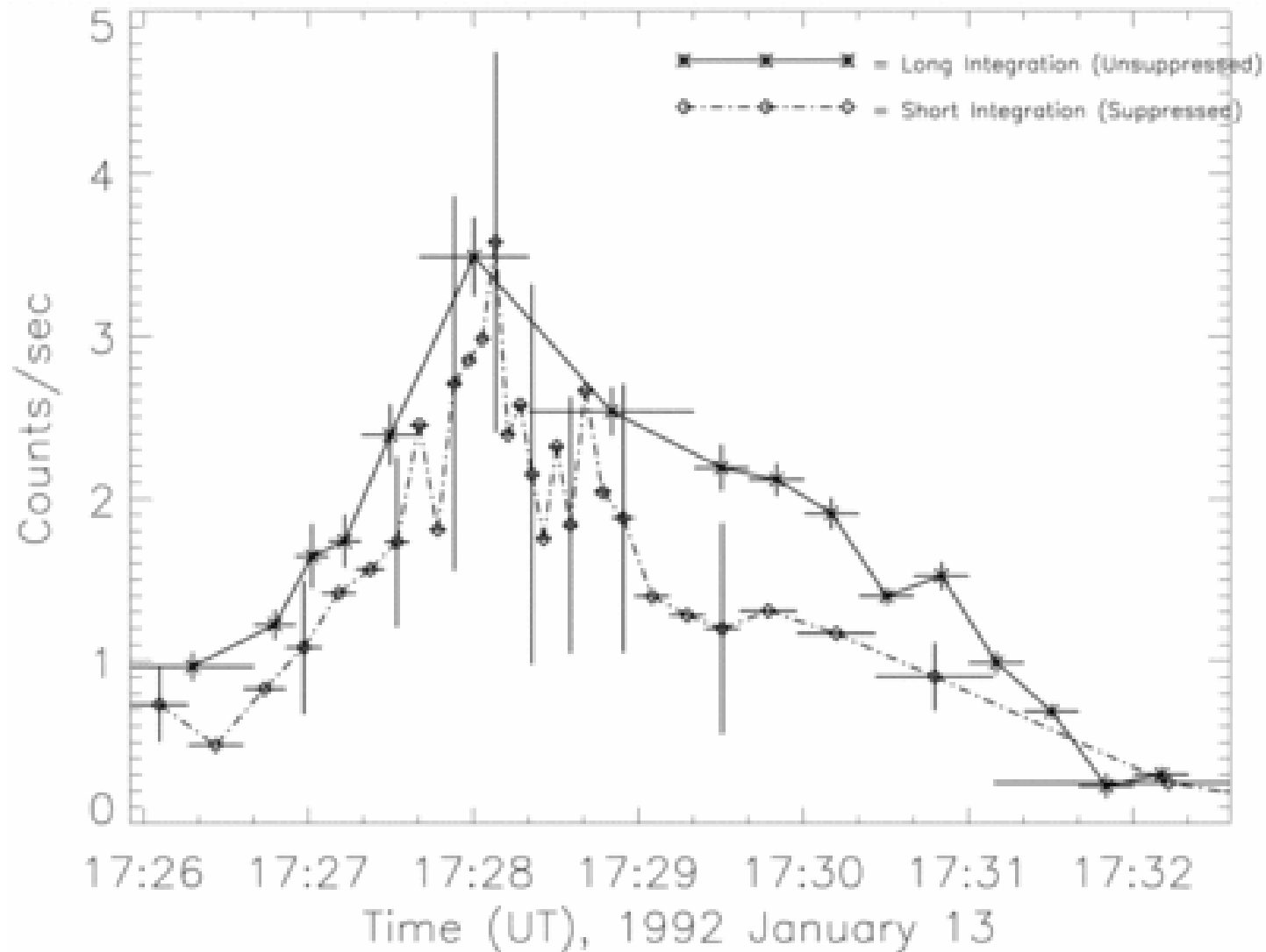
Fig. 6. from A Spectral Analysis of the Masuda Flare Using Yohkoh Hard XRay Telescope Pixon Reconstruction Alexander & Metcalf 1997 ApJ 489 442 doi:10.1086/304762 https://dx.doi.org/10.1086/304762 © 1997. The American Astronomical Society. All rights reserved. Printed in U.S.A.
