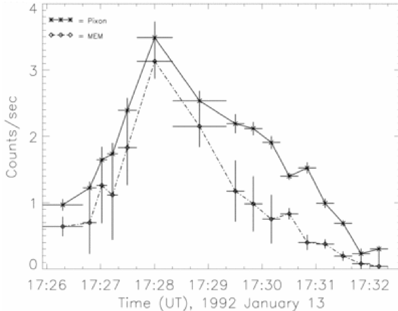
Fig. 5. from A Spectral Analysis of the Masuda Flare Using Yohkoh Hard XRay Telescope Pixon Reconstruction Alexander & Metcalf 1997 ApJ 489 442 doi:10.1086/304762 https://dx.doi.org/10.1086/304762 © 1997. The American Astronomical Society. All rights reserved. Printed in U.S.A.
