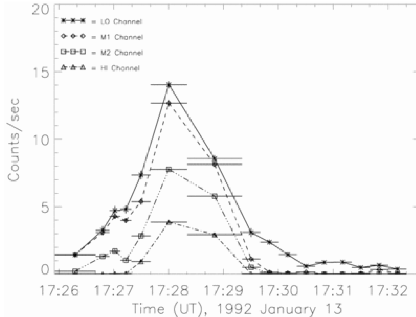
Fig. 3. from A Spectral Analysis of the Masuda Flare Using Yohkoh Hard XRay Telescope Pixon Reconstruction Alexander & Metcalf 1997 ApJ 489 442 doi:10.1086/304762 https://dx.doi.org/10.1086/304762 © 1997. The American Astronomical Society. All rights reserved. Printed in U.S.A.
