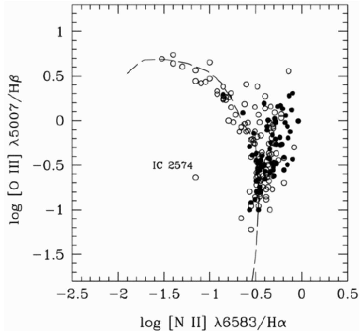
Fig. 9. from Properties of H II Regions in the Centers of Nearby Galaxies Ho, Filippenko, & Sargent 1997 ApJ 487 579 doi:10.1086/304642 https://dx.doi.org/10.1086/304642 © 1997. The American Astronomical Society. All rights reserved. Printed in U.S.A.
