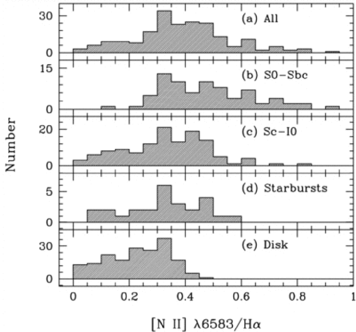
Fig. 8. from Properties of H II Regions in the Centers of Nearby Galaxies Ho, Filippenko, & Sargent 1997 ApJ 487 579 doi:10.1086/304642 https://dx.doi.org/10.1086/304642 © 1997. The American Astronomical Society. All rights reserved. Printed in U.S.A.
