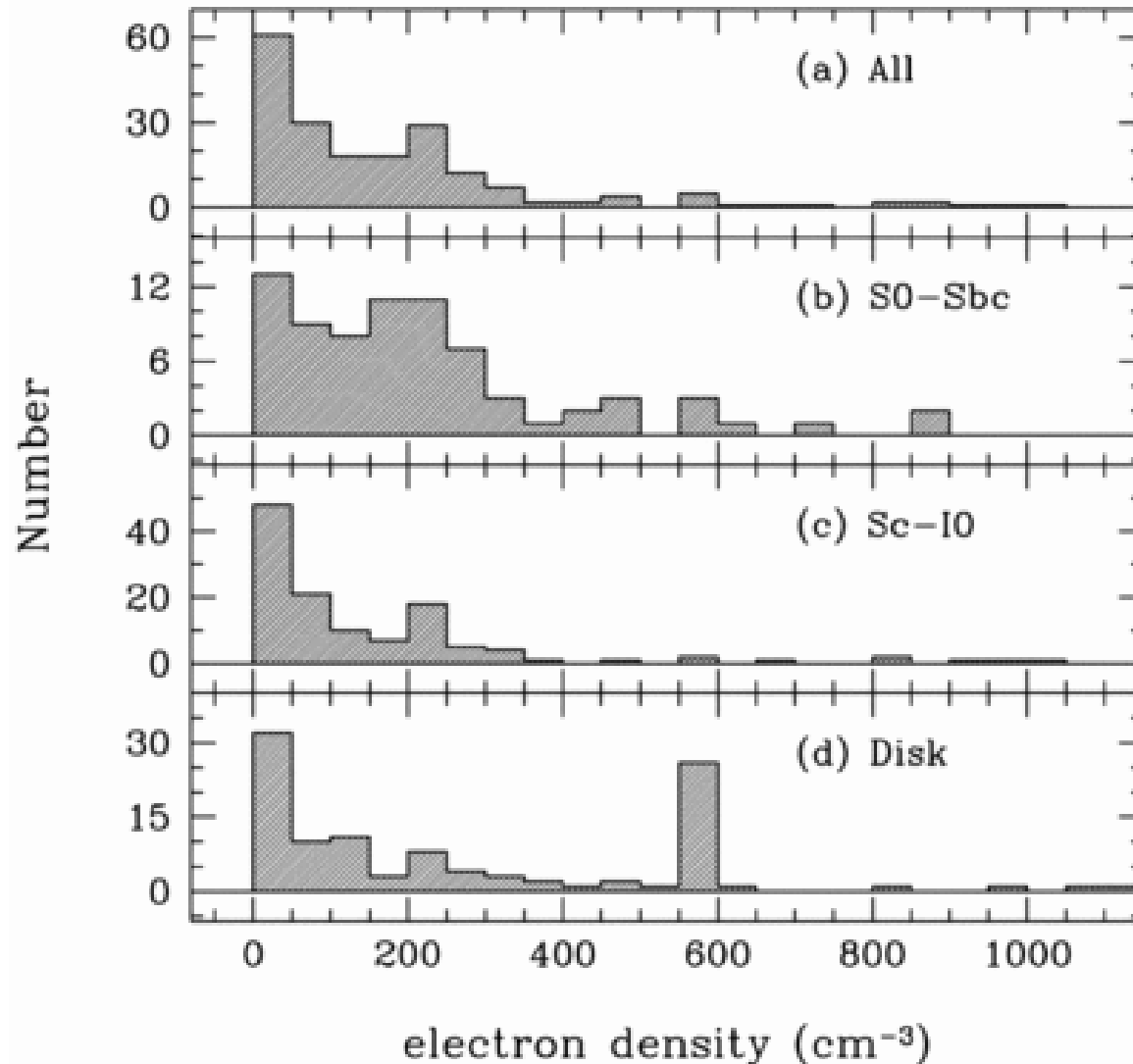
Fig. 5. from Properties of H II Regions in the Centers of Nearby Galaxies Ho, Filippenko, & Sargent 1997 ApJ 487 579 doi:10.1086/304642 https://dx.doi.org/10.1086/304642 © 1997. The American Astronomical Society. All rights reserved. Printed in U.S.A.
