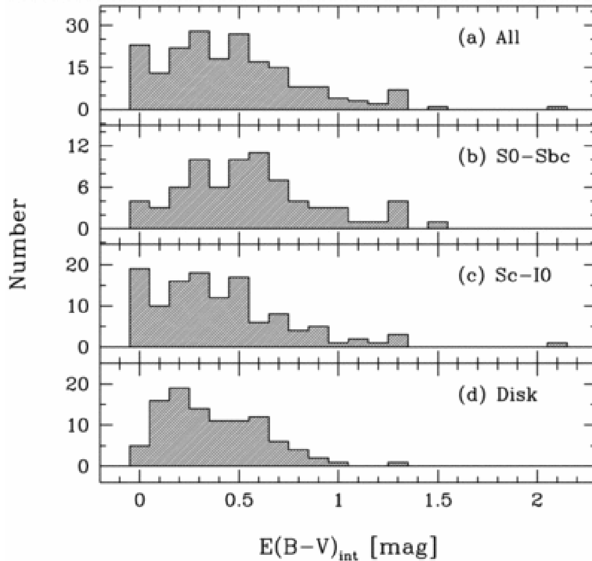
Fig. 4. from Properties of H II Regions in the Centers of Nearby Galaxies Ho, Filippenko, & Sargent 1997 ApJ 487 579 doi:10.1086/304642 https://dx.doi.org/10.1086/304642 © 1997. The American Astronomical Society. All rights reserved. Printed in U.S.A.
