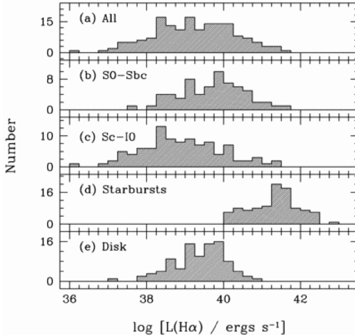
Fig. 2. from Properties of H II Regions in the Centers of Nearby Galaxies Ho, Filippenko, & Sargent 1997 ApJ 487 579 doi:10.1086/304642 https://dx.doi.org/10.1086/304642 © 1997. The American Astronomical Society. All rights reserved. Printed in U.S.A.
