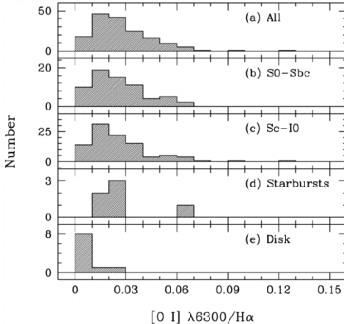
Fig. 13. from Properties of H II Regions in the Centers of Nearby Galaxies Ho, Filippenko, & Sargent 1997 ApJ 487 579 doi:10.1086/304642 https://dx.doi.org/10.1086/304642 © 1997. The American Astronomical Society. All rights reserved. Printed in U.S.A.
