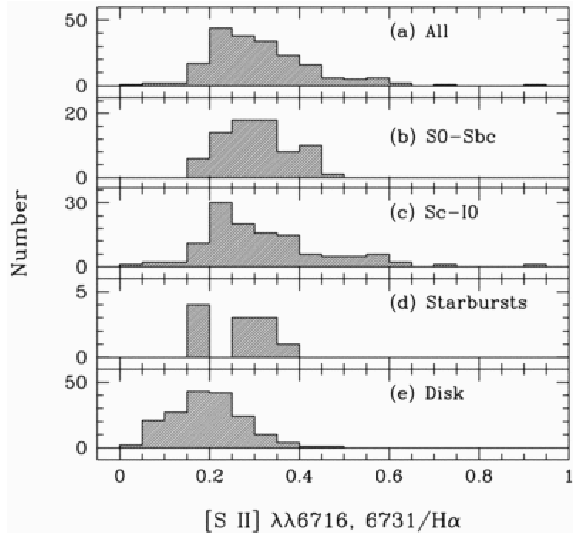
Fig. 11. from Properties of H II Regions in the Centers of Nearby Galaxies Ho, Filippenko, & Sargent 1997 ApJ 487 579 doi:10.1086/304642 https://dx.doi.org/10.1086/304642 © 1997. The American Astronomical Society. All rights reserved. Printed in U.S.A.
