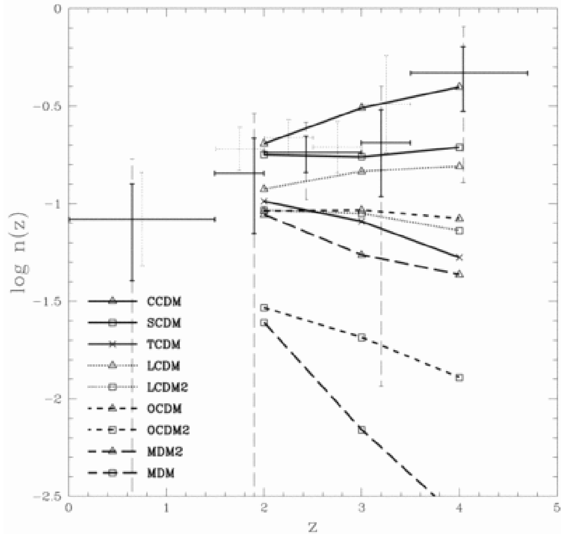
Fig. 1. from Testing Cosmological Models against the Abundance of Damped LymanAlpha Absorbers Gardner et al. 1997 ApJ 486 42 doi:10.1086/304526 https://dx.doi.org/10.1086/304526 © 1997. The American Astronomical Society. All rights reserved. Printed in U.S.A.
