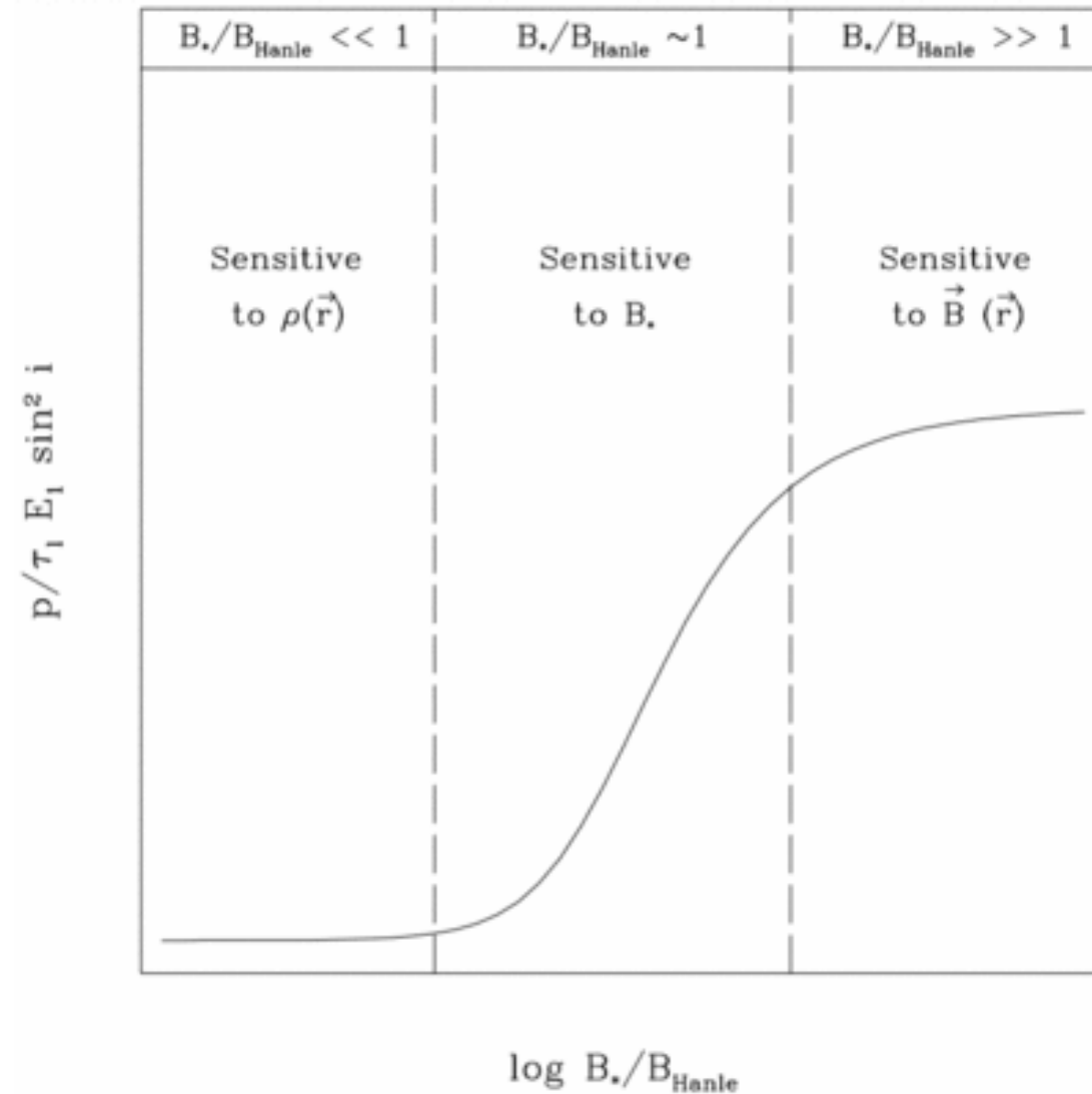
Fig. 7. from The Hanle Effect as a Diagnostic of Magnetic Fields in Stellar Envelopes. I. Theoretical Results for Integrated Line Profiles Ignace, Nordsieck, & Cassinelli 1997 ApJ 486 550 doi:10.1086/304512 https://dx.doi.org/10.1086/304512 © 1997. The American Astronomical Society. All rights reserved. Printed in U.S.A.
