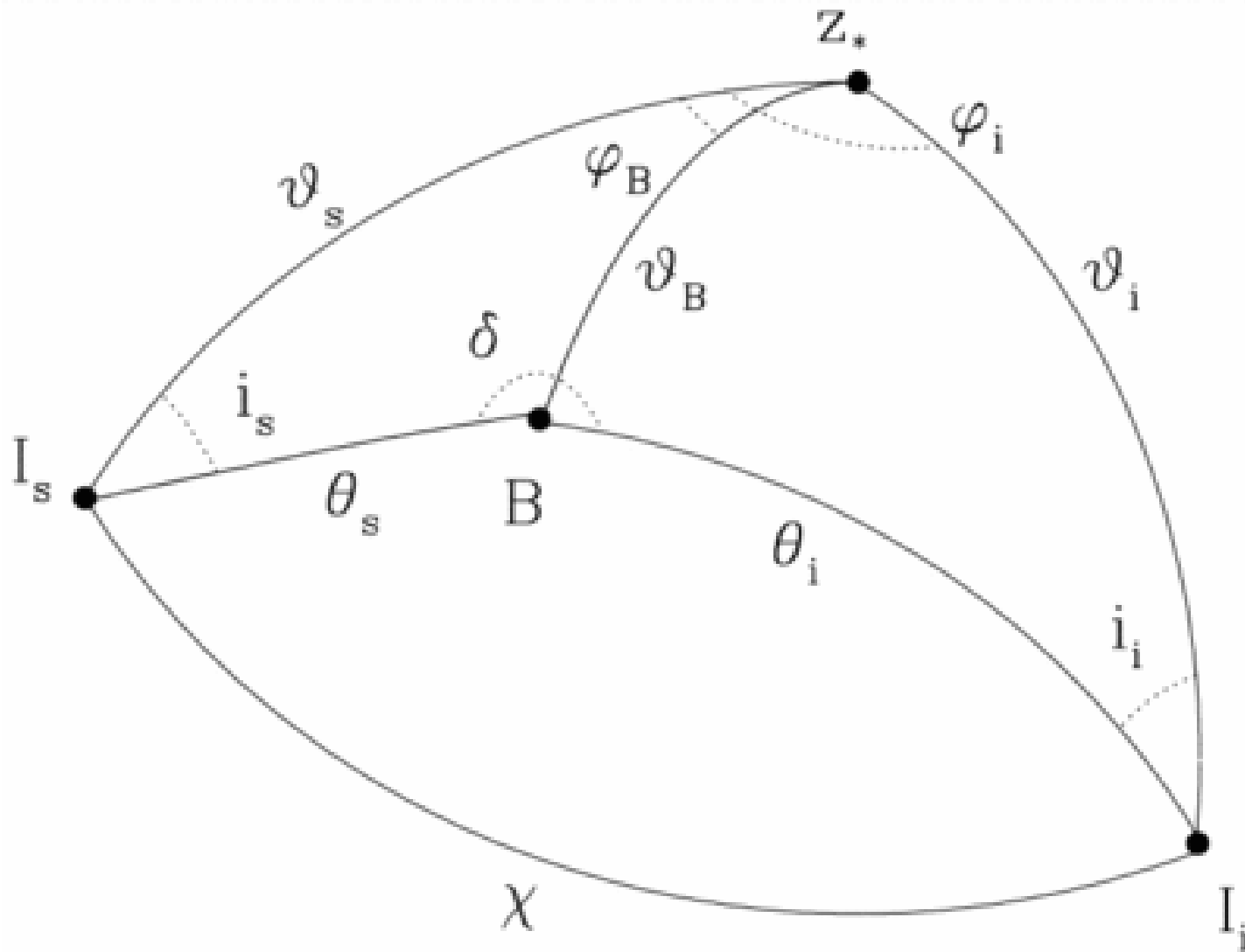
Fig. 4. from The Hanle Effect as a Diagnostic of Magnetic Fields in Stellar Envelopes. I. Theoretical Results for Integrated Line Profiles Ignace, Nordsieck, & Cassinelli 1997 ApJ 486 550 doi:10.1086/304512 https://dx.doi.org/10.1086/304512 © 1997. The American Astronomical Society. All rights reserved. Printed in U.S.A.
