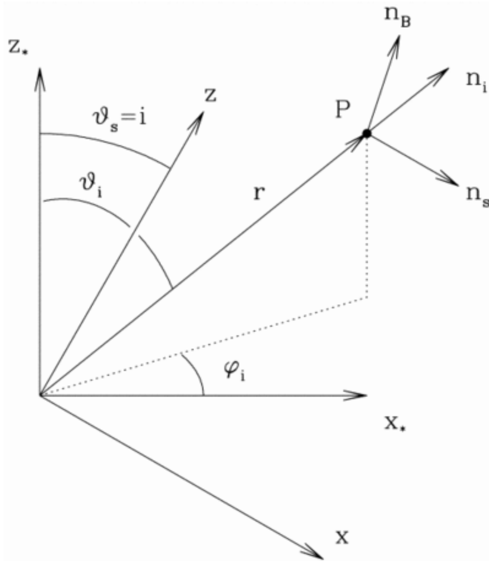
Fig. 3. from The Hanle Effect as a Diagnostic of Magnetic Fields in Stellar Envelopes. I. Theoretical Results for Integrated Line Profiles Ignace, Nordsieck, & Cassinelli 1997 ApJ 486 550 doi:10.1086/304512 https://dx.doi.org/10.1086/304512 © 1997. The American Astronomical Society. All rights reserved. Printed in U.S.A.
