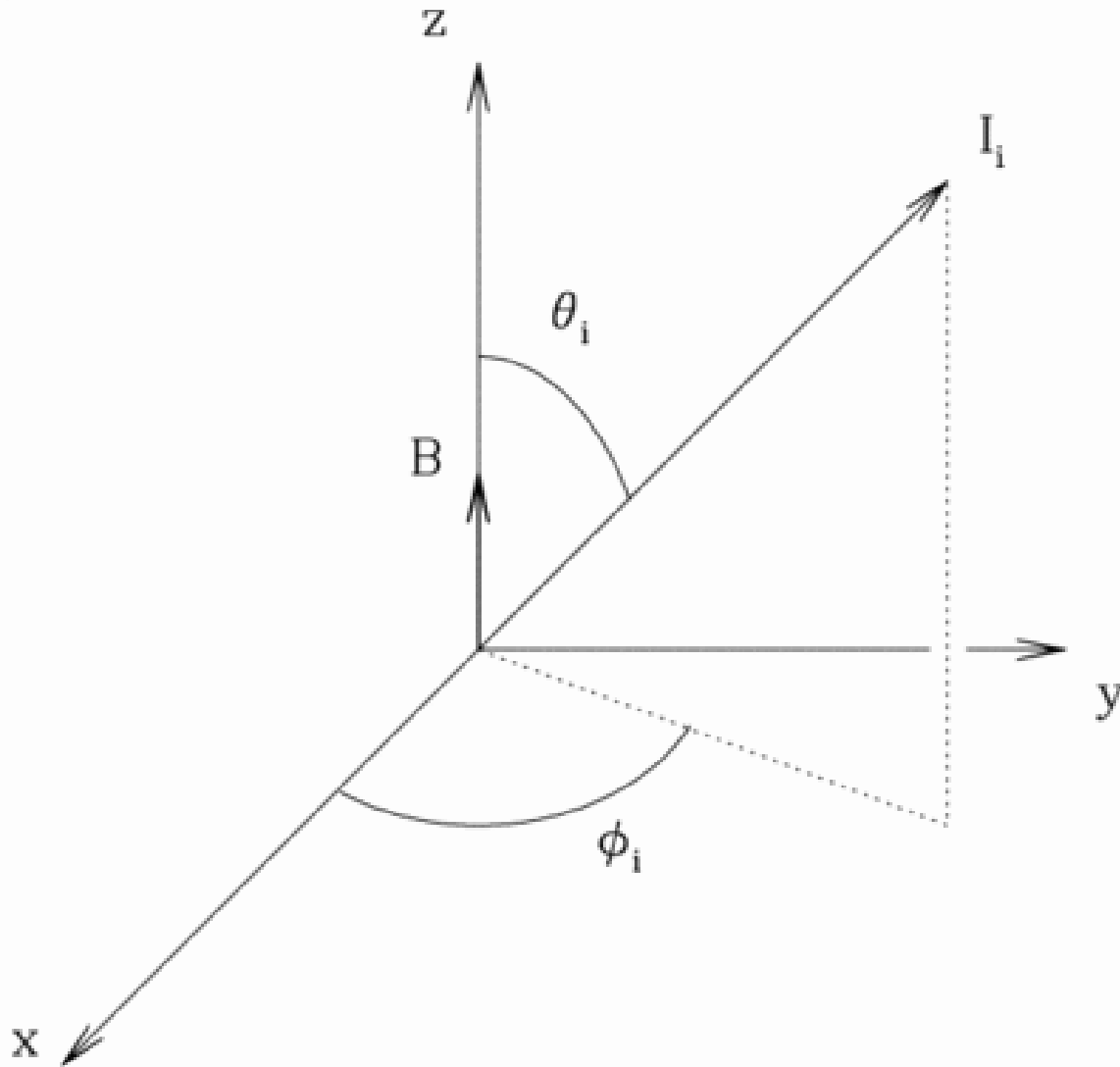
Fig. 2. from The Hanle Effect as a Diagnostic of Magnetic Fields in Stellar Envelopes. I. Theoretical Results for Integrated Line Profiles Ignace, Nordsieck, & Cassinelli 1997 ApJ 486 550 doi:10.1086/304512 https://dx.doi.org/10.1086/304512 © 1997. The American Astronomical Society. All rights reserved. Printed in U.S.A.
