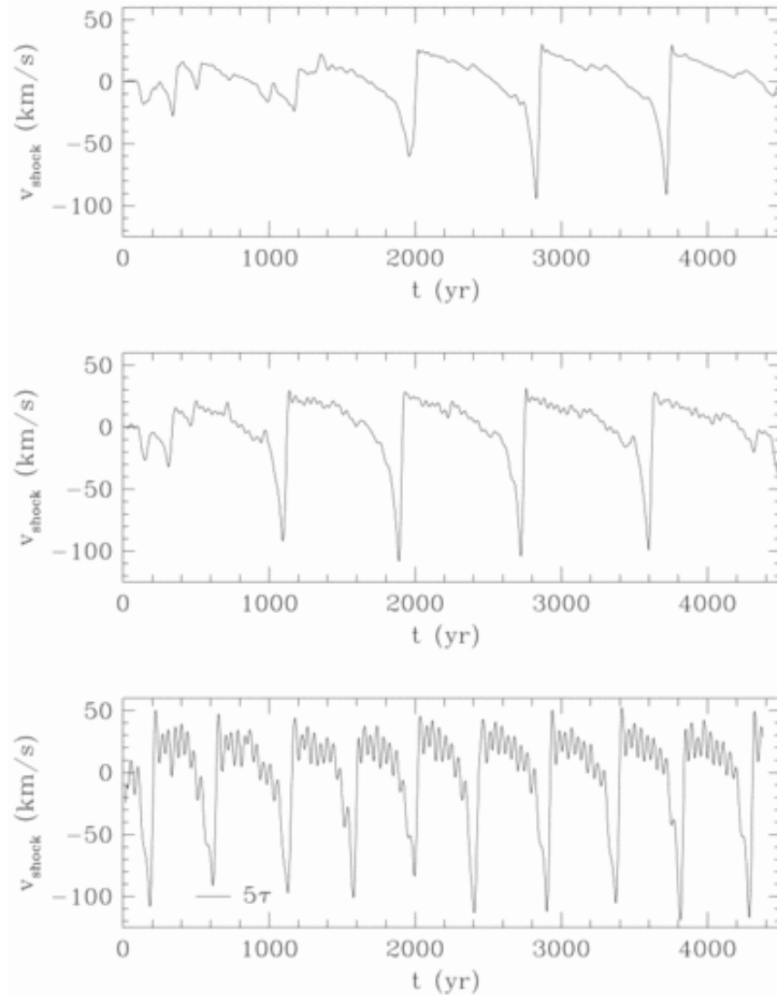
Fig. 9. from Radiative Instabilities in Simulations of Spherically Symmetric Supernova Blast Waves Kimoto & Chernoff 1997 ApJ 485 274 doi:10.1086/304408 https://dx.doi.org/10.1086/304408 © 1997. The American Astronomical Society. All rights reserved. Printed in U.S.A.
