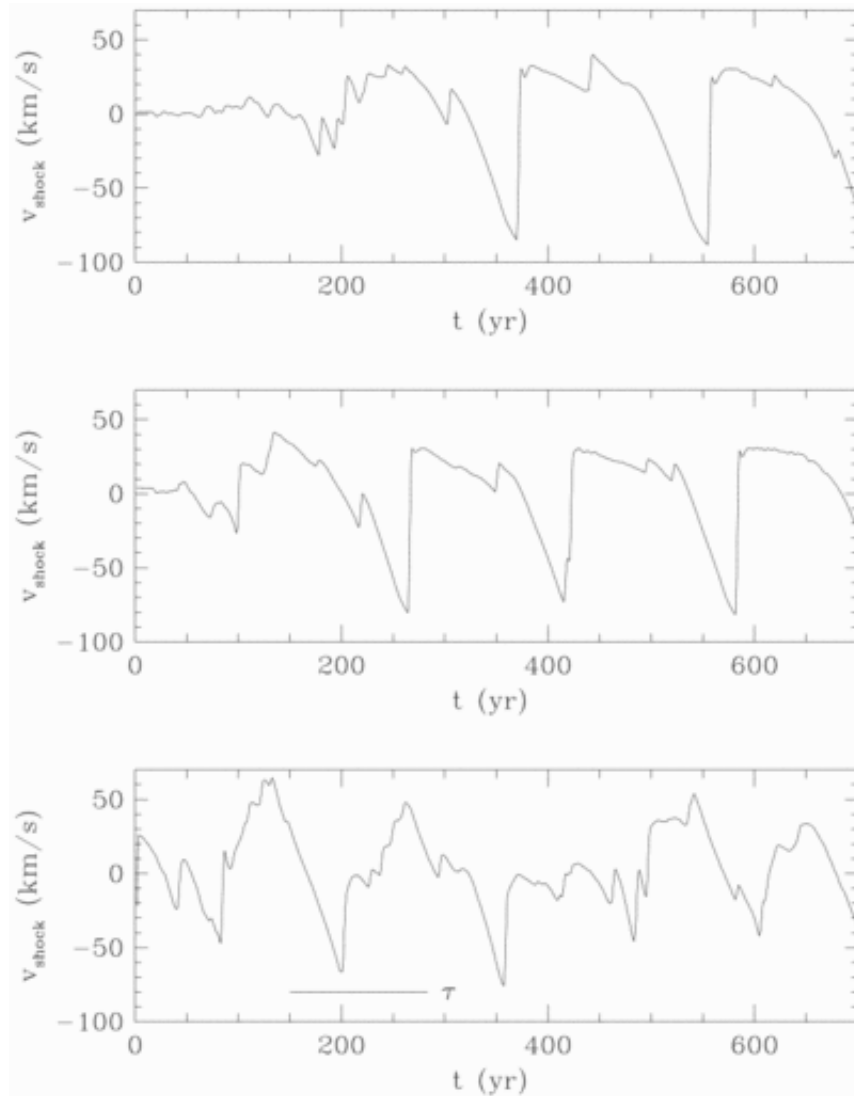
Fig. 8. from Radiative Instabilities in Simulations of Spherically Symmetric Supernova Blast Waves Kimoto & Chernoff 1997 ApJ 485 274 doi:10.1086/304408 https://dx.doi.org/10.1086/304408 © 1997. The American Astronomical Society. All rights reserved. Printed in U.S.A.
