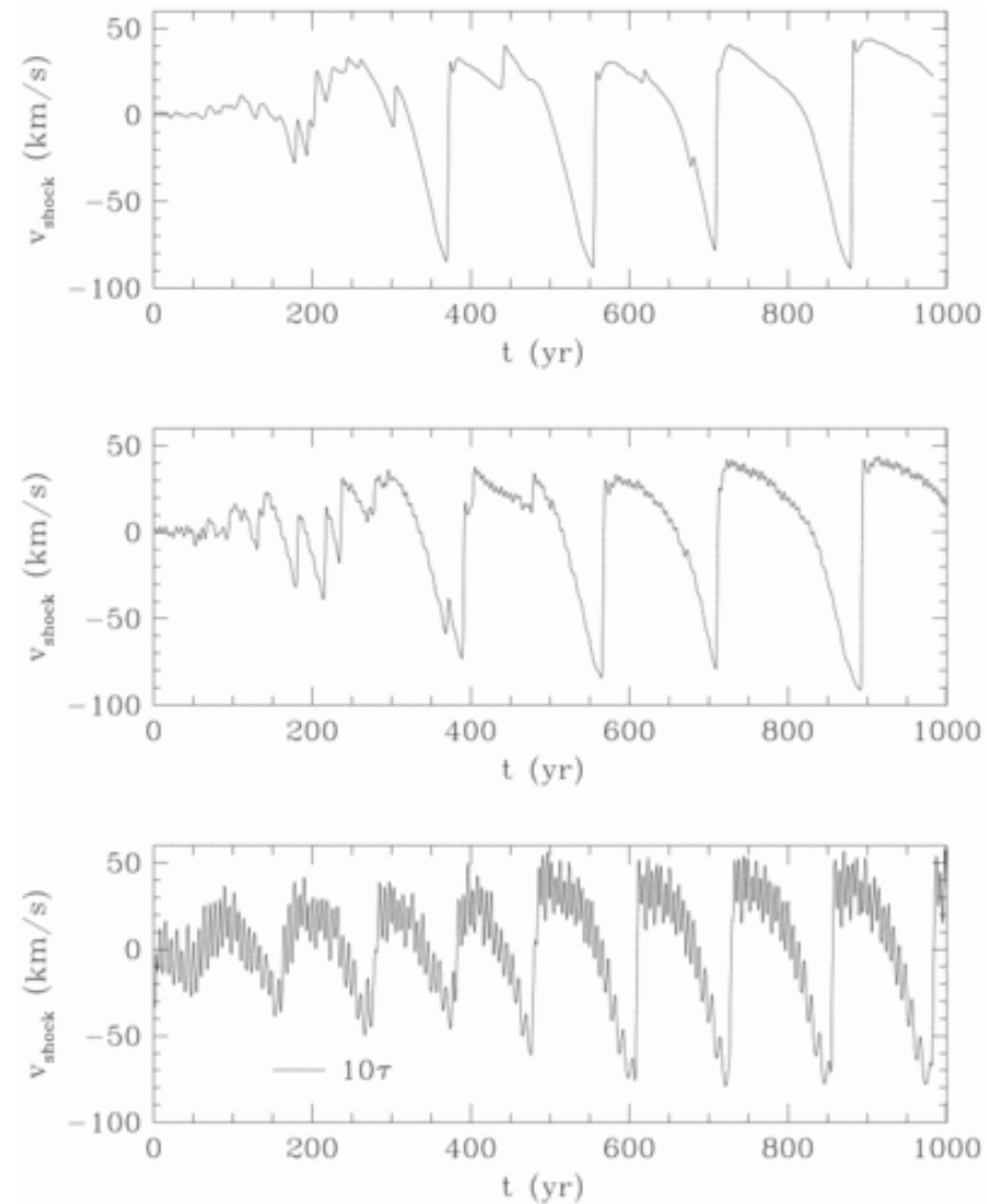
Fig. 7. from Radiative Instabilities in Simulations of Spherically Symmetric Supernova Blast Waves Kimoto & Chernoff 1997 ApJ 485 274 doi:10.1086/304408 https://dx.doi.org/10.1086/304408 © 1997. The American Astronomical Society. All rights reserved. Printed in U.S.A.
