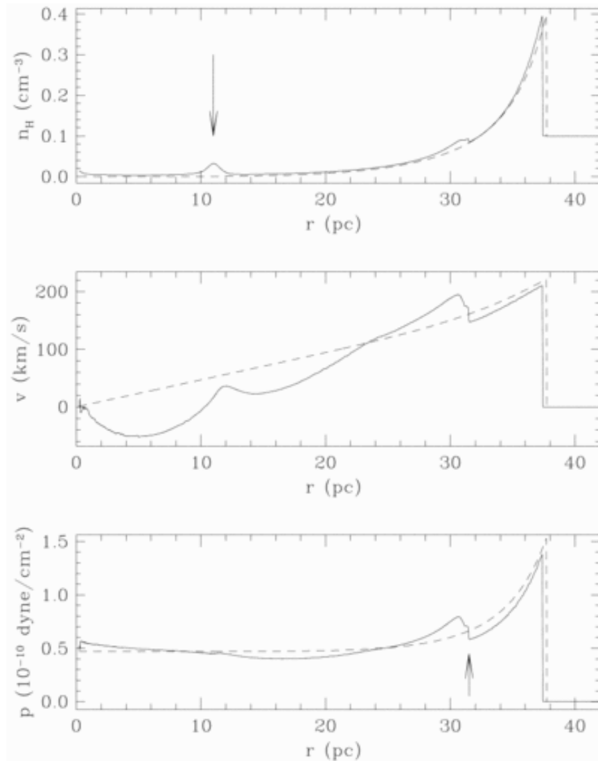
Fig. 6. from Radiative Instabilities in Simulations of Spherically Symmetric Supernova Blast Waves Kimoto & Chernoff 1997 ApJ 485 274 doi:10.1086/304408 https://dx.doi.org/10.1086/304408 © 1997. The American Astronomical Society. All rights reserved. Printed in U.S.A.
