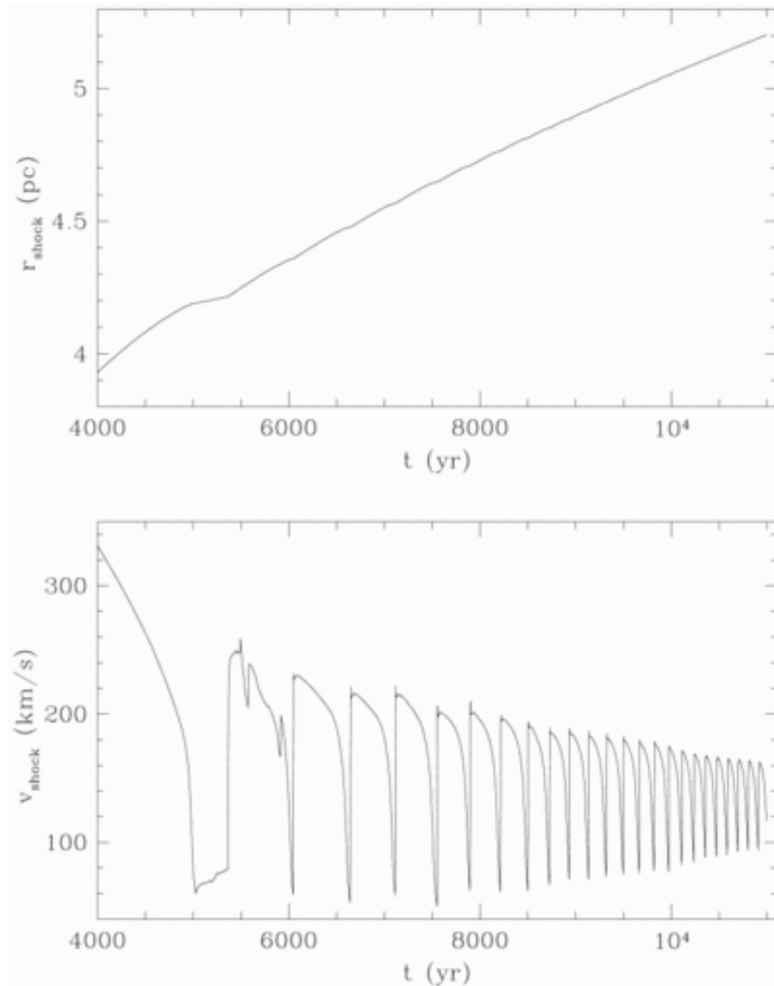
Fig. 4. from Radiative Instabilities in Simulations of Spherically Symmetric Supernova Blast Waves Kimoto & Chernoff 1997 ApJ 485 274 doi:10.1086/304408 https://dx.doi.org/10.1086/304408 © 1997. The American Astronomical Society. All rights reserved. Printed in U.S.A.
