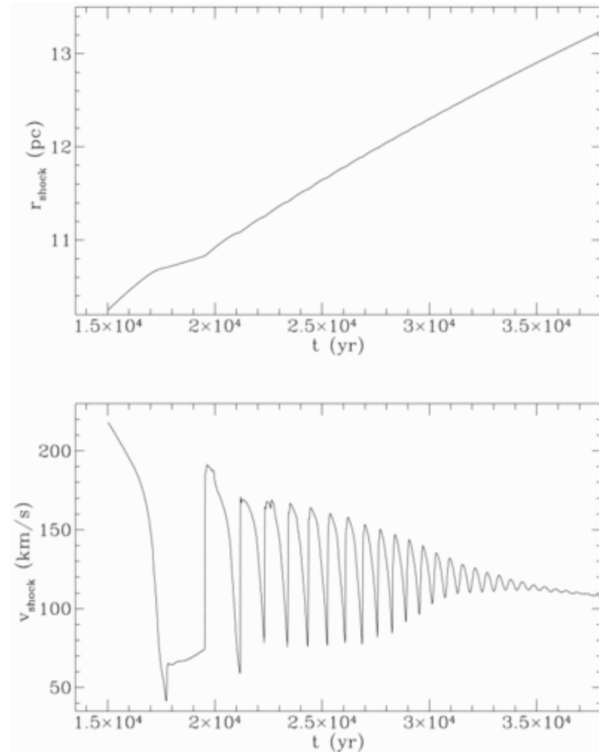
Fig. 3. from Radiative Instabilities in Simulations of Spherically Symmetric Supernova Blast Waves Kimoto & Chernoff 1997 ApJ 485 274 doi:10.1086/304408 https://dx.doi.org/10.1086/304408 © 1997. The American Astronomical Society. All rights reserved. Printed in U.S.A.
