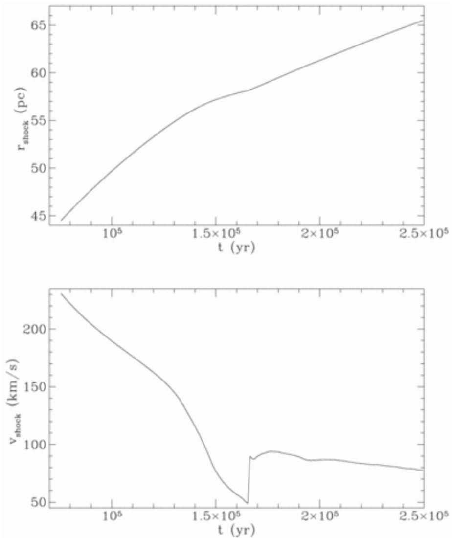
Fig. 2. from Radiative Instabilities in Simulations of Spherically Symmetric Supernova Blast Waves Kimoto & Chernoff 1997 ApJ 485 274 doi:10.1086/304408 https://dx.doi.org/10.1086/304408 © 1997. The American Astronomical Society. All rights reserved. Printed in U.S.A.
