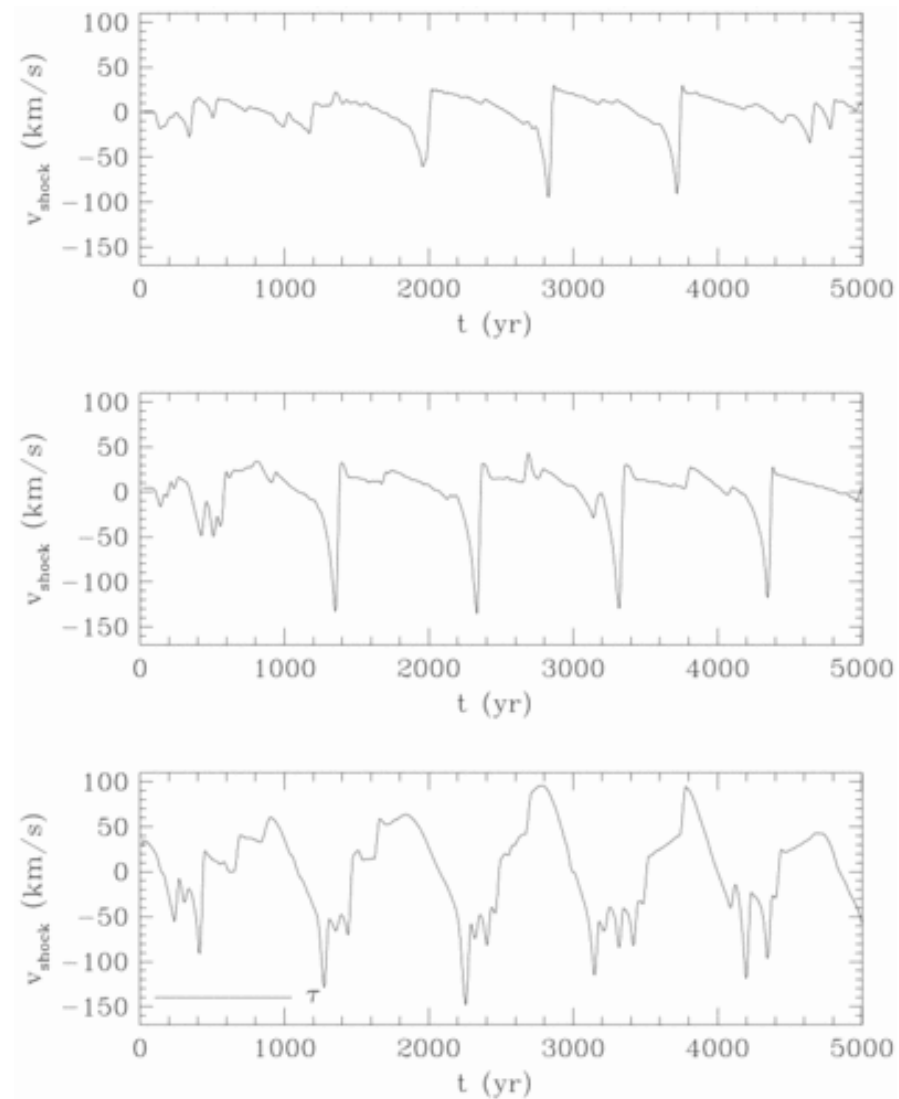
Fig. 10. from Radiative Instabilities in Simulations of Spherically Symmetric Supernova Blast Waves Kimoto & Chernoff 1997 ApJ 485 274 doi:10.1086/304408 https://dx.doi.org/10.1086/304408 © 1997. The American Astronomical Society. All rights reserved. Printed in U.S.A.
