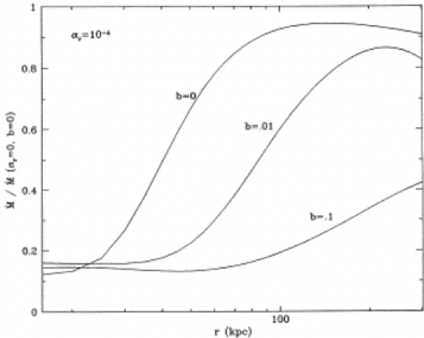
Fig. 5. from A Feedback Model for Radio Sources Fueled by Cooling Flows Tucker & David 1997 ApJ 484 602 doi:10.1086/304345 https://dx.doi.org/10.1086/304345 © 1997. The American Astronomical Society. All rights reserved. Printed in U.S.A.
